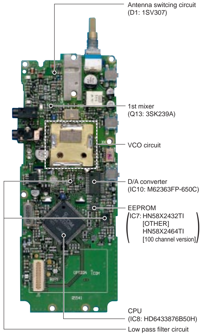
BOTTOM VIEW
